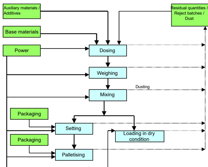
Fig. 1: Manufacturing process (green: input; blue: uniform process)
