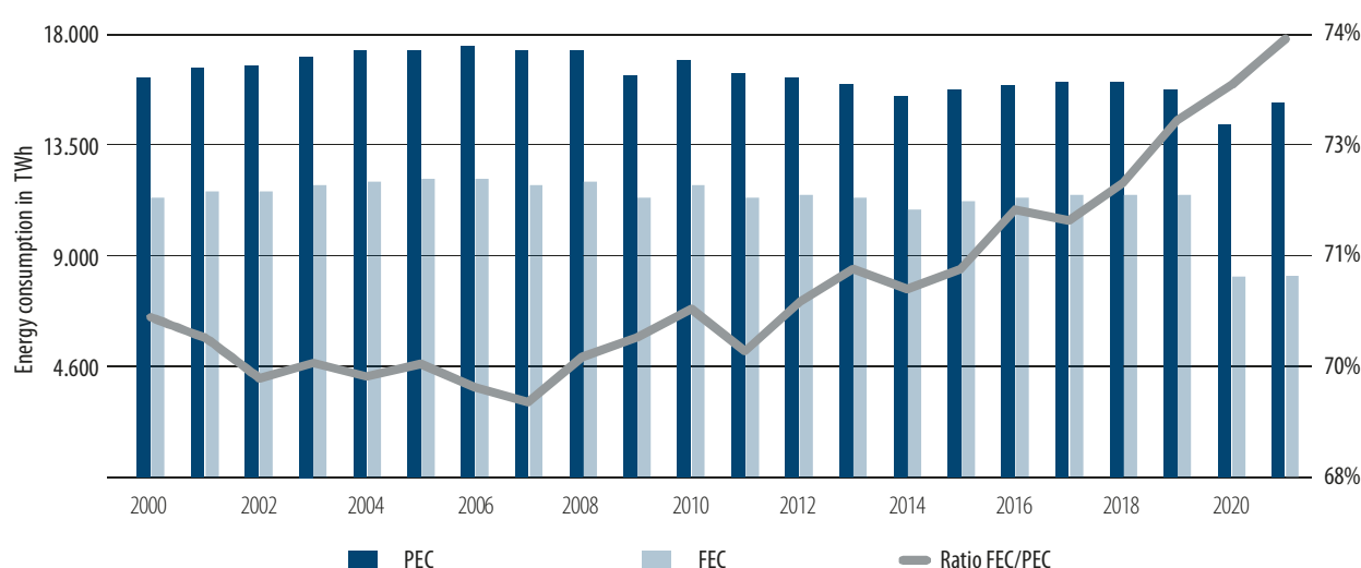
Primary energy consumption (PEC), final energy consumption (FEC) and the ratio of FEC to PEC in EU from 2000 – 2021
