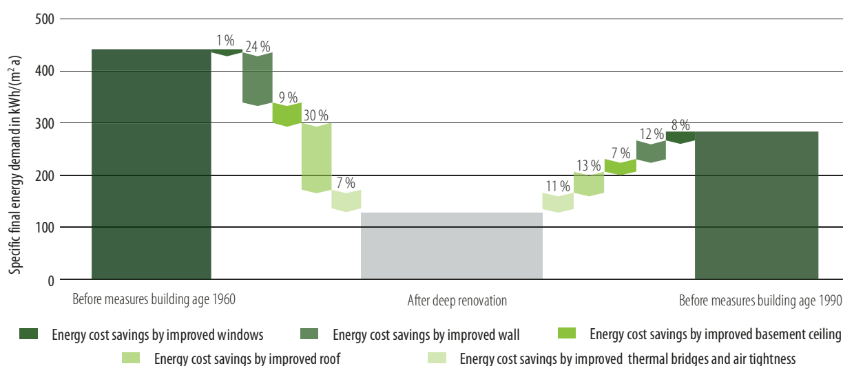
Figure 26 Energy cost savings by component-improvements compared to two initial states Source: FIW
