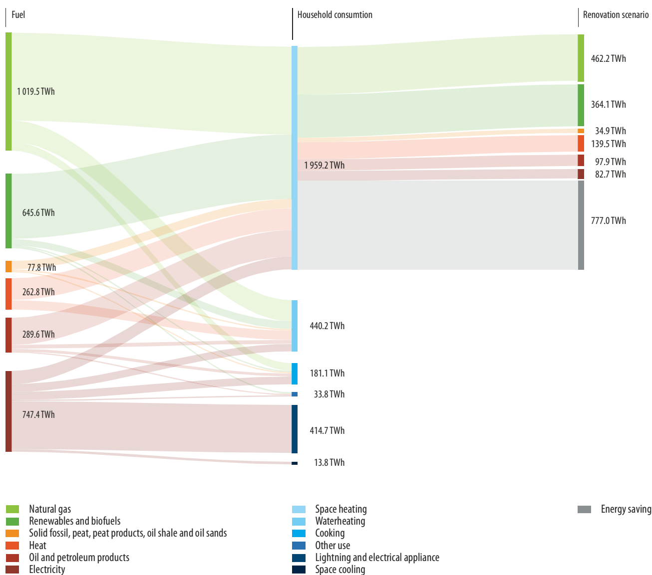
Figure 37 Energy consumption in EU household by fuel, 2021. *Renovation of walls and roofs of EU's residential buildings. Source: Eurostat (nrg_d_hhq) and BPIE [58]
