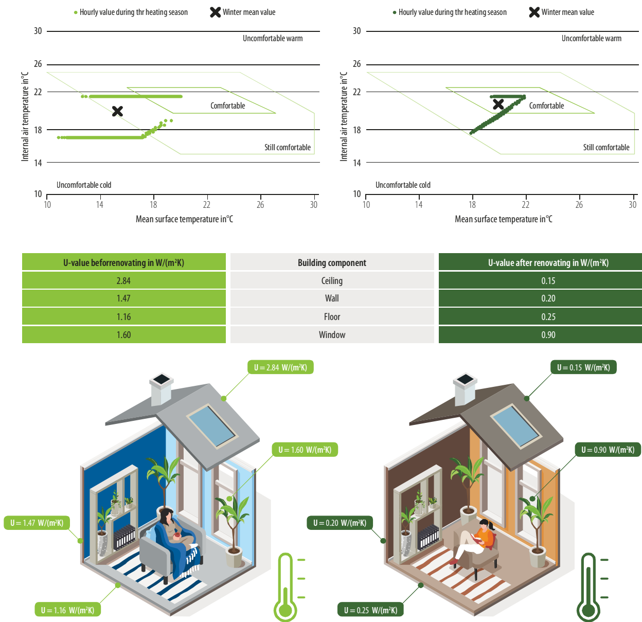
Figure 25 1) Thermal comfort in a single-family-house built in 1960; 2) Thermal comfort in a single-family-house built in 1960 after renovation. Source: FIW
