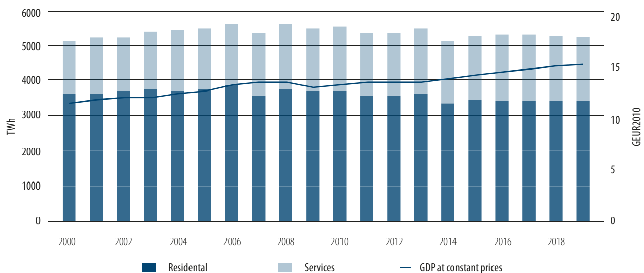
Figure 5 Total final energy consumption for the EU building stock and GDP. Source: Odysee [17]
