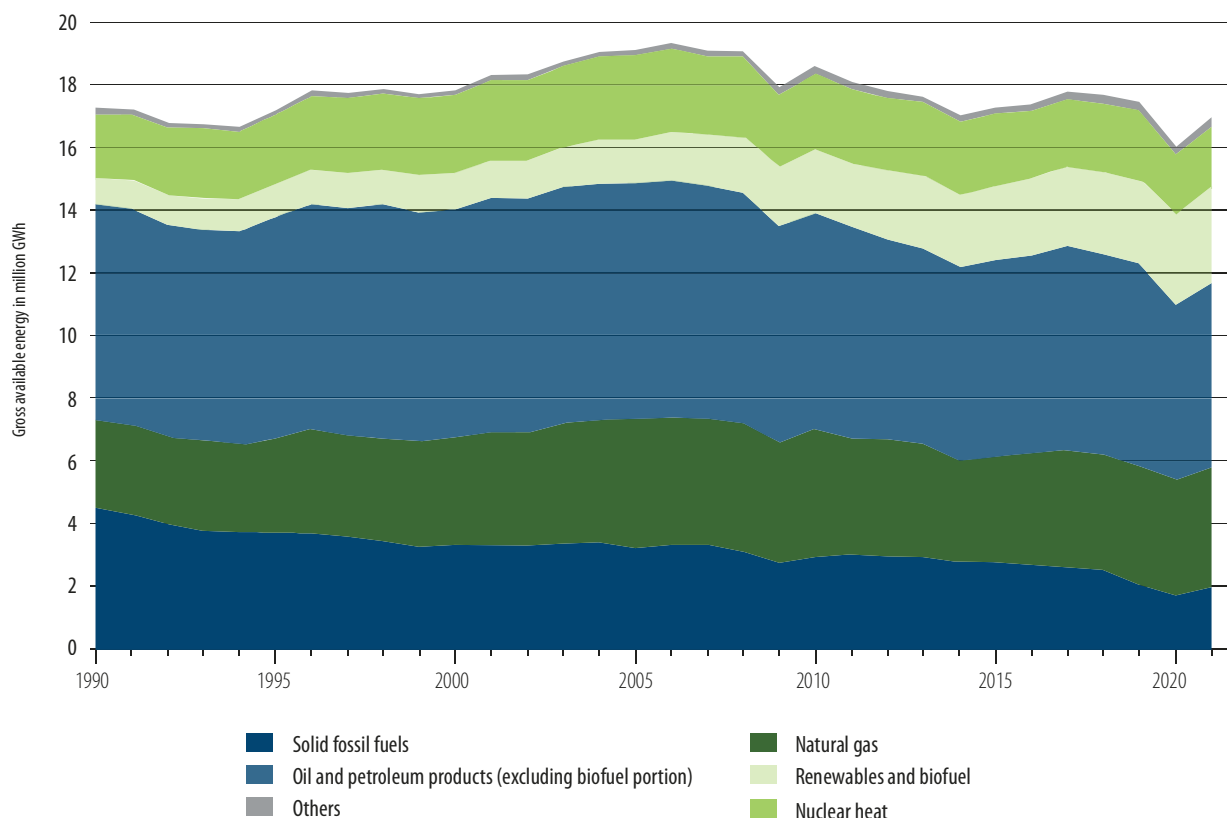
Figure 32 Gross available energy by fuel in GWh in EU - 27 countries from 1990 until 2021. Source: Eurostat (nrg_bal_c)
