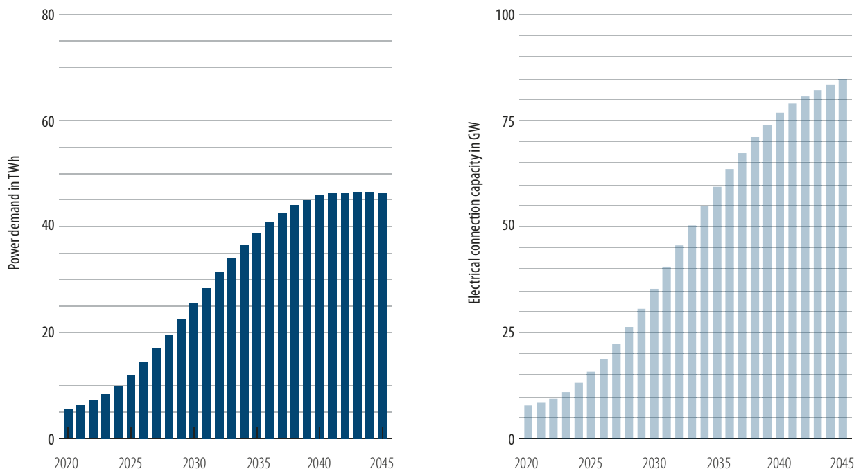
Figure 7 Forecast of heat pumps' electricity demand and heating load for residential buildings in Germany until 2045. Source: FIW
