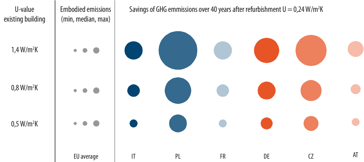
Comparison of effort and achievable GHG savings over 40 years for refurbishment to a U-value of 0.24 W/(m²·K) for various existing situations.
